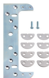
Kit reinforcing plate with spacers and screws for cover frame
